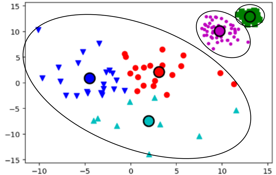
k-means (5 Clusters)
